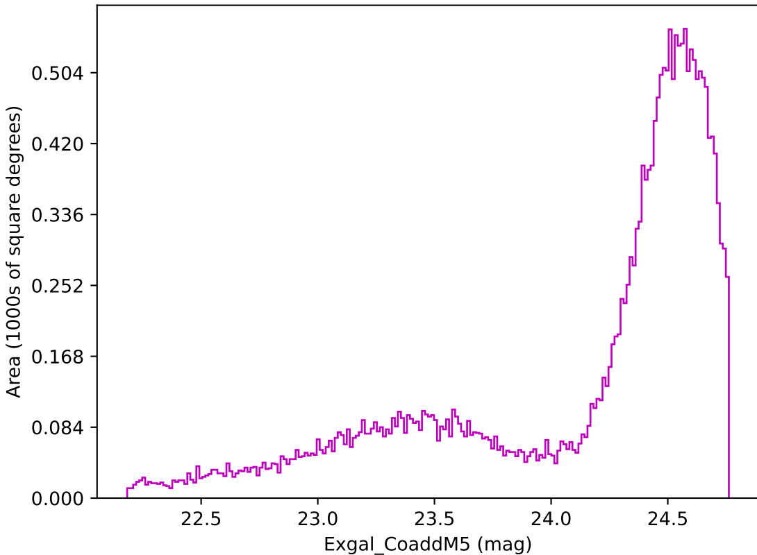
too_ignore_100_1v3.4_10yrs Yr 1 z band: Exgal_CoaddM5
