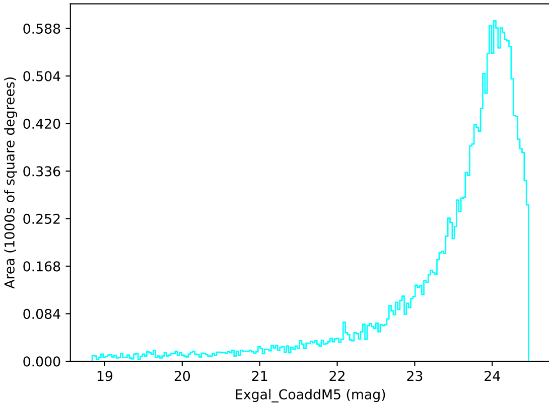
too_ignore_100_1v3.4_10yrs Yr 1 u band: Exgal_CoaddM5
