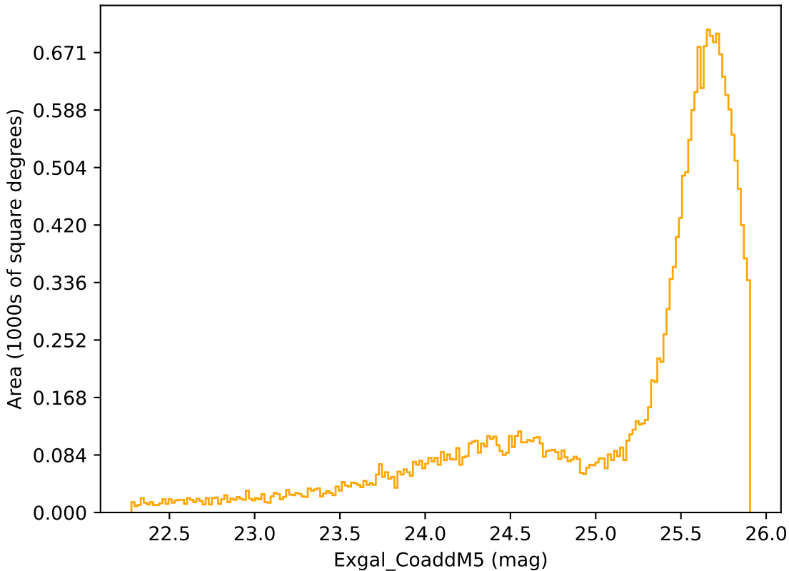
too_ignore_100_1v3.4_10yrs Yr 1 r band: Exgal_CoaddM5
