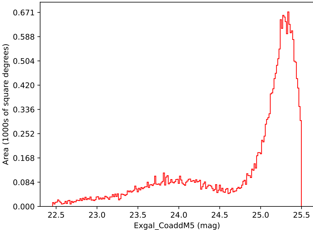
too_ignore_100_1v3.4_10yrs Yr 1 i band: Exgal_CoaddM5
