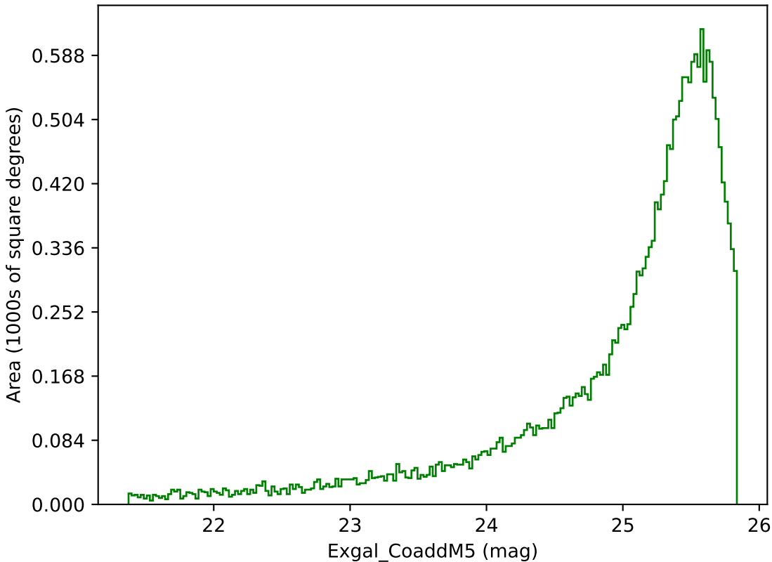
too_ignore_100_1v3.4_10yrs Yr 1 g band: Exgal_CoaddM5
