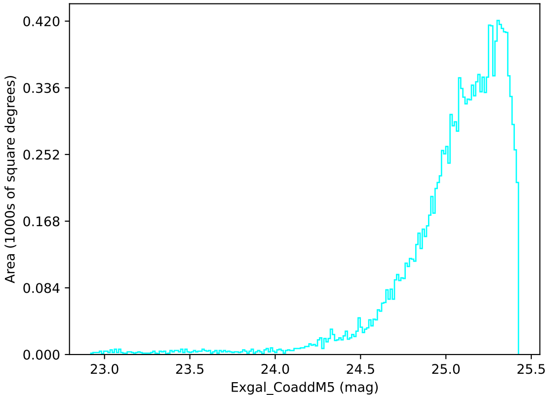
too_ignore_100_1v3.4_10yrs WFD u band: Exgal_CoaddM5
