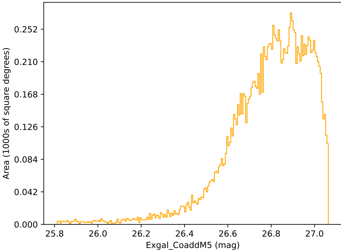
too_ignore_100_1v3.4_10yrs WFD r band: Exgal_CoaddM5
