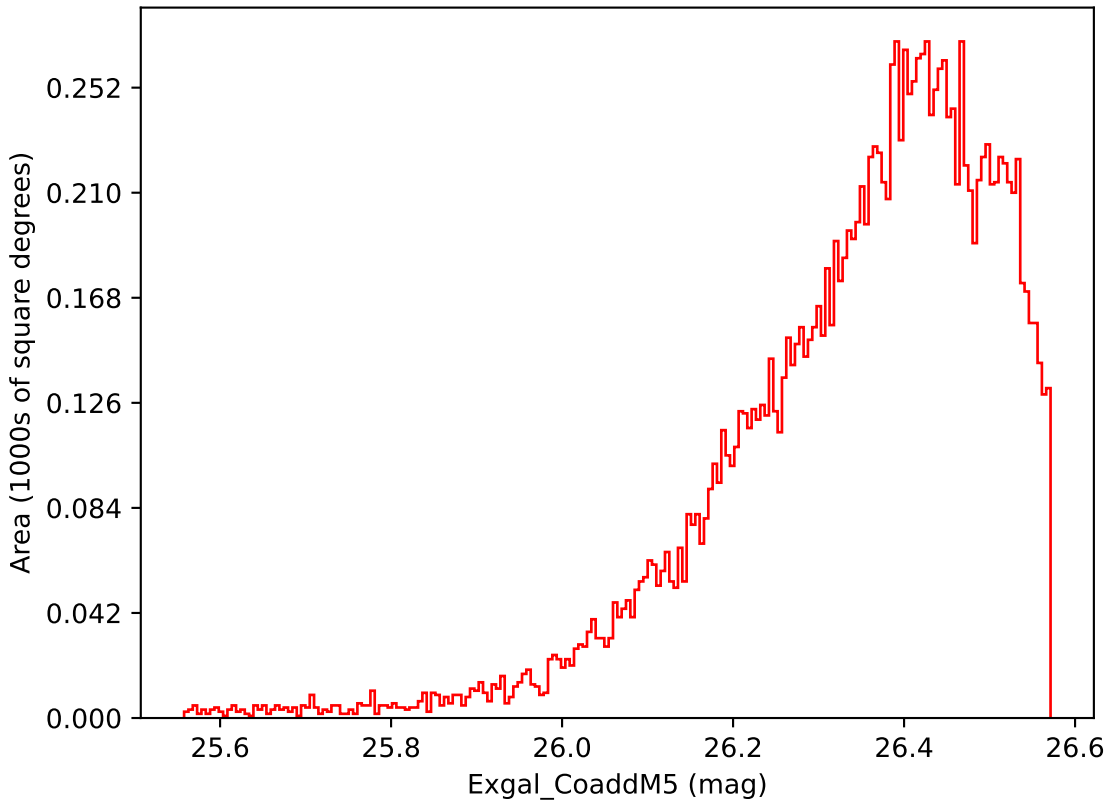
too_ignore_100_1v3.4_10yrs WFD i band: Exgal_CoaddM5
