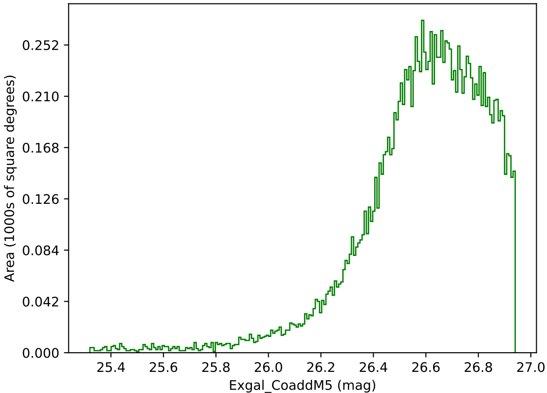
too_ignore_100_1v3.4_10yrs WFD g band: Exgal_CoaddM5
