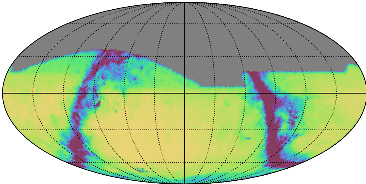
too_ignore_100_1v3.4_10yrs All sky g band: Exgal_CoaddM5
