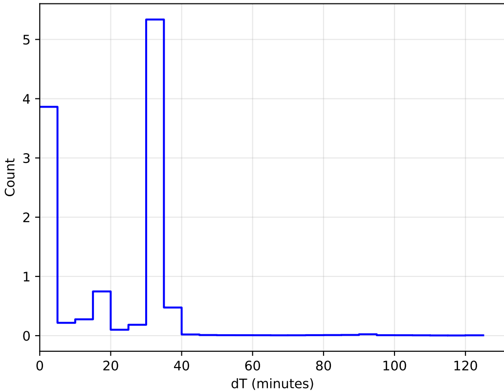
1e6 too_ignore_100_1v3.4_10yrs WFD: DeltaT Histogram
