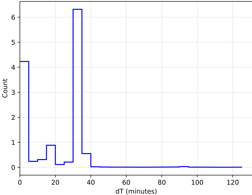
too_ignore_100_1v3.4_10yrs All sky: DeltaT Histogram
