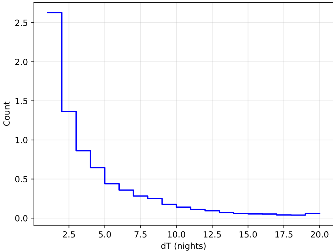
too_ignore_100_1v3.4_10yrs WFD all bands: DeltaNight Histogram 1e6
