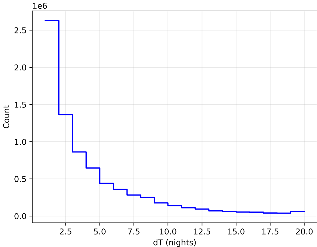
too_ignore_100_1v3.4_10yrs WFD all bands: DeltaNight Histogram
