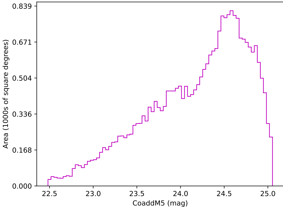
too_ignore_100_1v3.4_10yrs Yr 3-4 z band: CoaddM5
