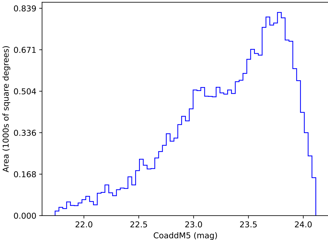
too_ignore_100_1v3.4_10yrs Yr 3-4 y band: CoaddM5
