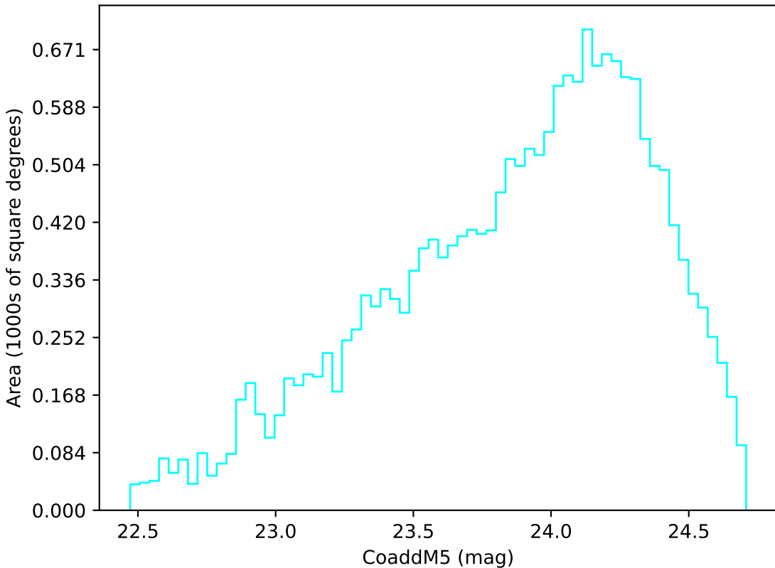
too_ignore_100_1v3.4_10yrs Yr 3-4 u band: CoaddM5
