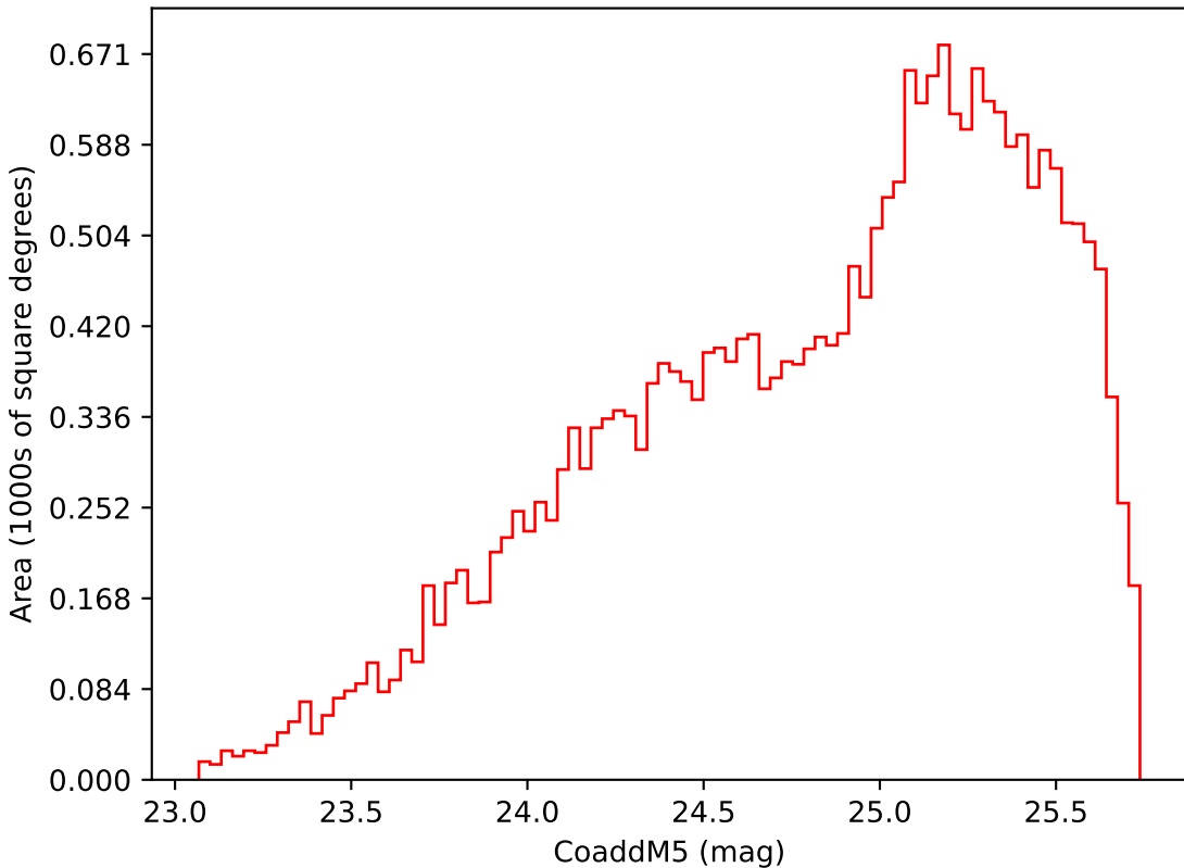
too_ignore_100_1v3.4_10yrs Yr 3-4 i band: CoaddM5
