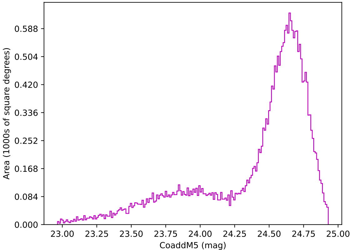
too_ignore_100_1v3.4_10yrs Yr 1 z band: CoaddM5
