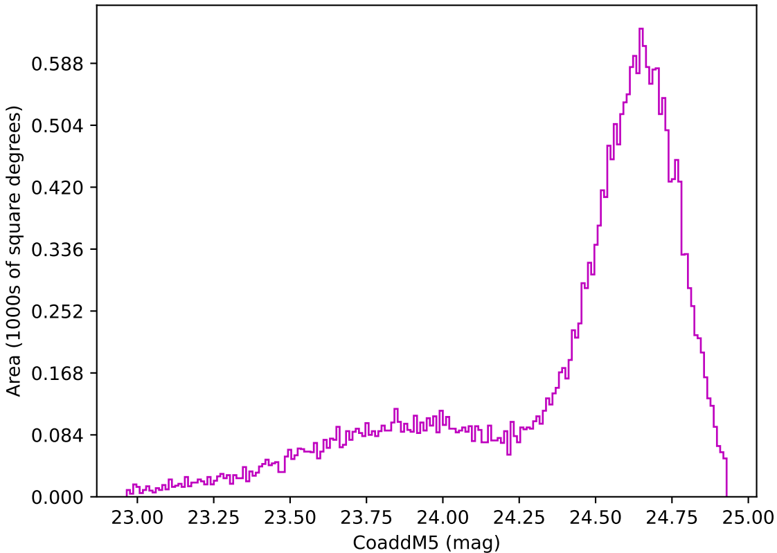
too_ignore_100_1v3.4_10yrs Yr 1 z band: CoaddM5
