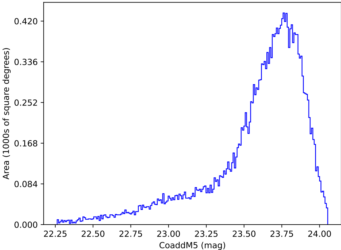
too_ignore_100_1v3.4_10yrs Yr 1 y band: CoaddM5
