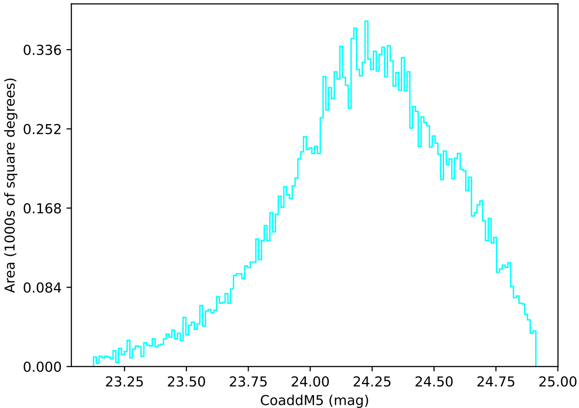
too_ignore_100_1v3.4_10yrs Yr 1 u band: CoaddM5
