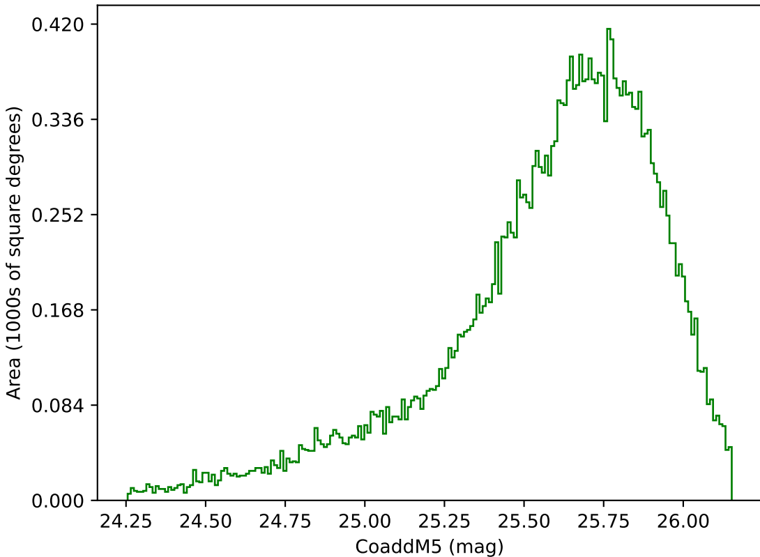
too_ignore_100_1v3.4_10yrs Yr 1 g band: CoaddM5
