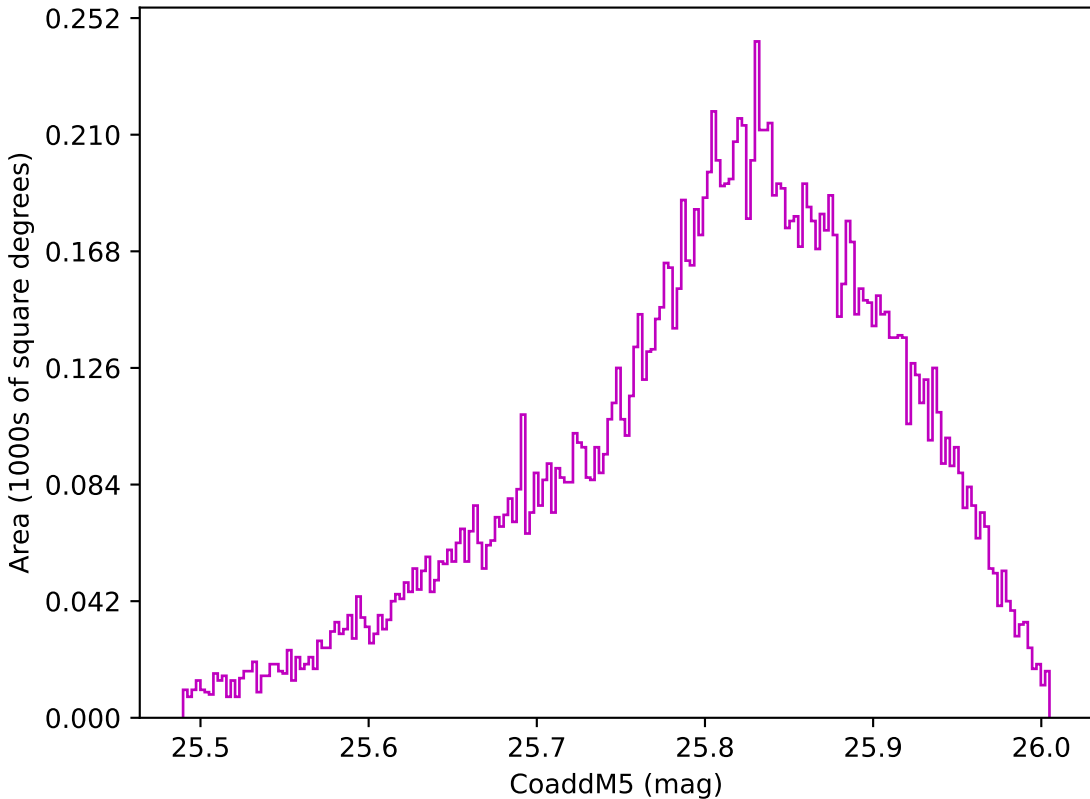
too_ignore_100_1v3.4_10yrs WFD z band: CoaddM5
