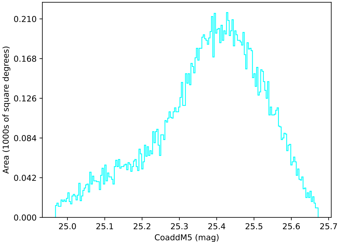
too_ignore_100_1v3.4_10yrs WFD u band: CoaddM5
