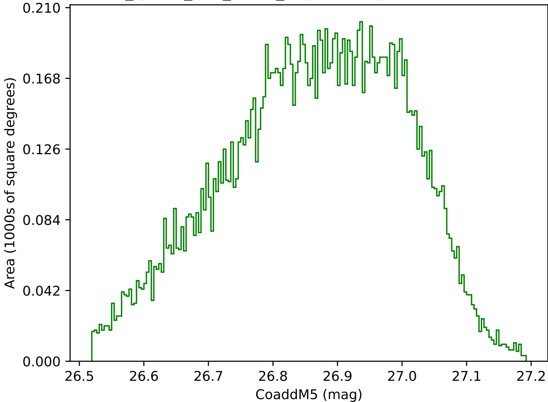
too_ignore_100_1v3.4_10yrs WFD g band: CoaddM5
