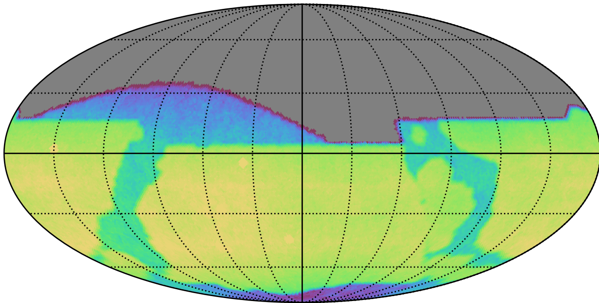
too_ignore_100_1v3.4_10yrs All sky z band: CoaddM5
