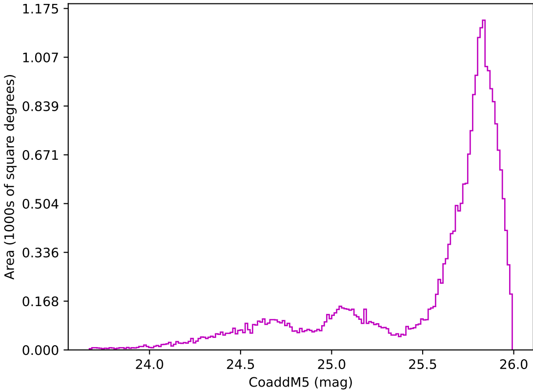
too_ignore_100_1v3.4_10yrs All sky z band: CoaddM5
