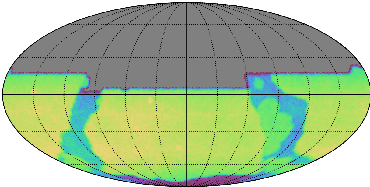
too_ignore_100_1v3.4_10yrs All sky y band: CoaddM5
