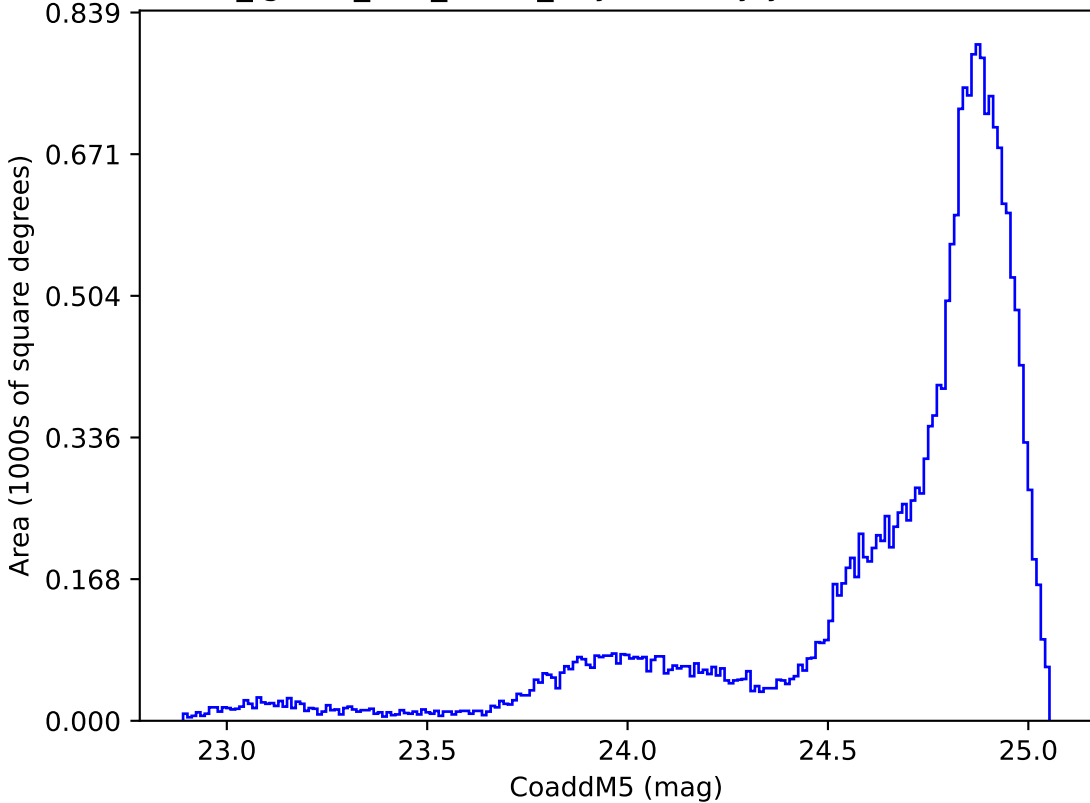
too_ignore_100_1v3.4_10yrs All sky y band: CoaddM5
