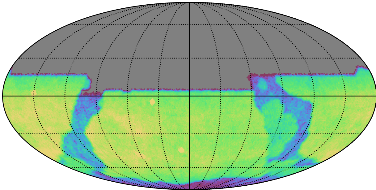
too_ignore_100_1v3.4_10yrs All sky u band: CoaddM5
