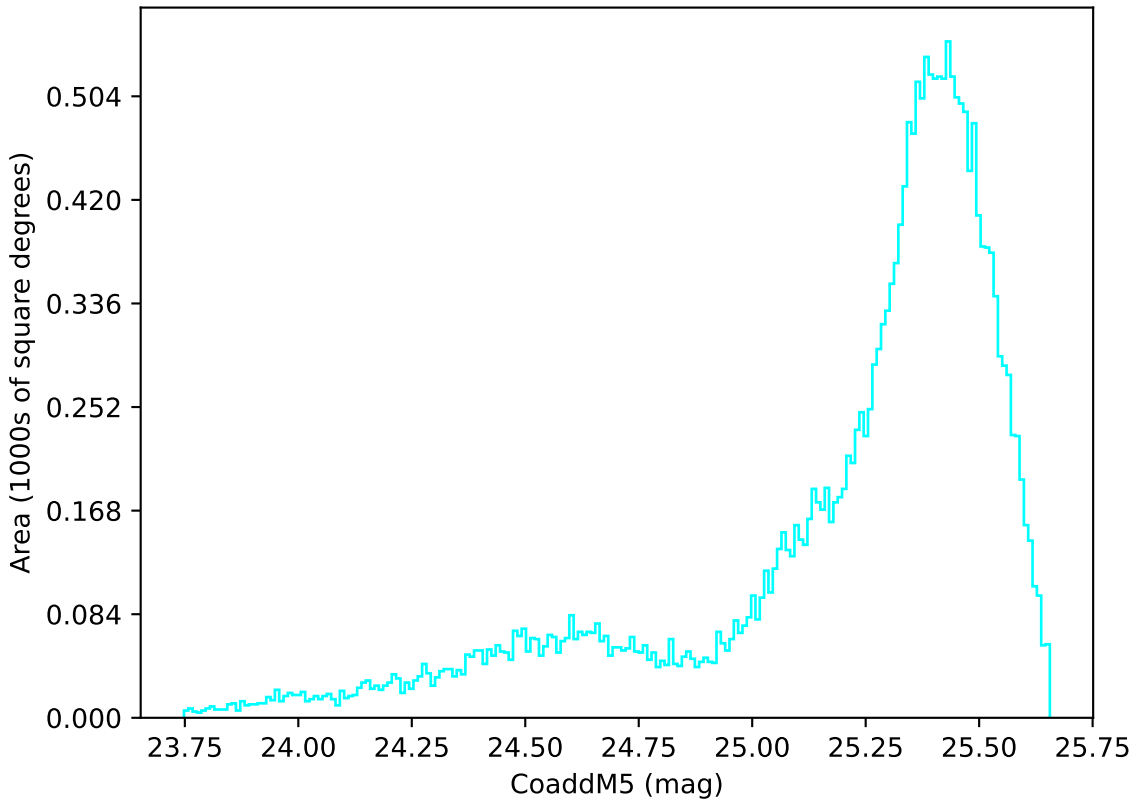
too_ignore_100_1v3.4_10yrs All sky u band: CoaddM5
