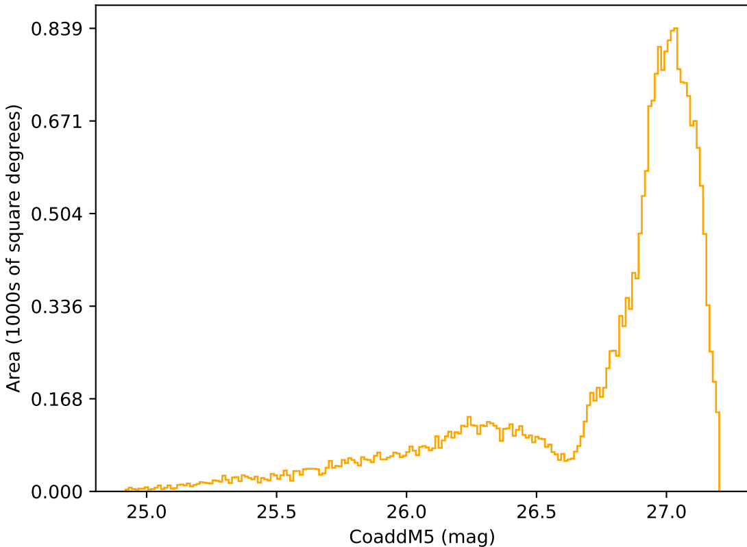
too_ignore_100_1v3.4_10yrs All sky r band: CoaddM5
