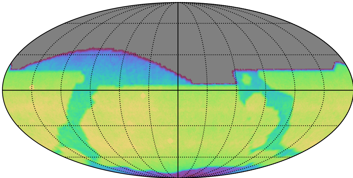
too_ignore_100_1v3.4_10yrs All sky i band: CoaddM5
