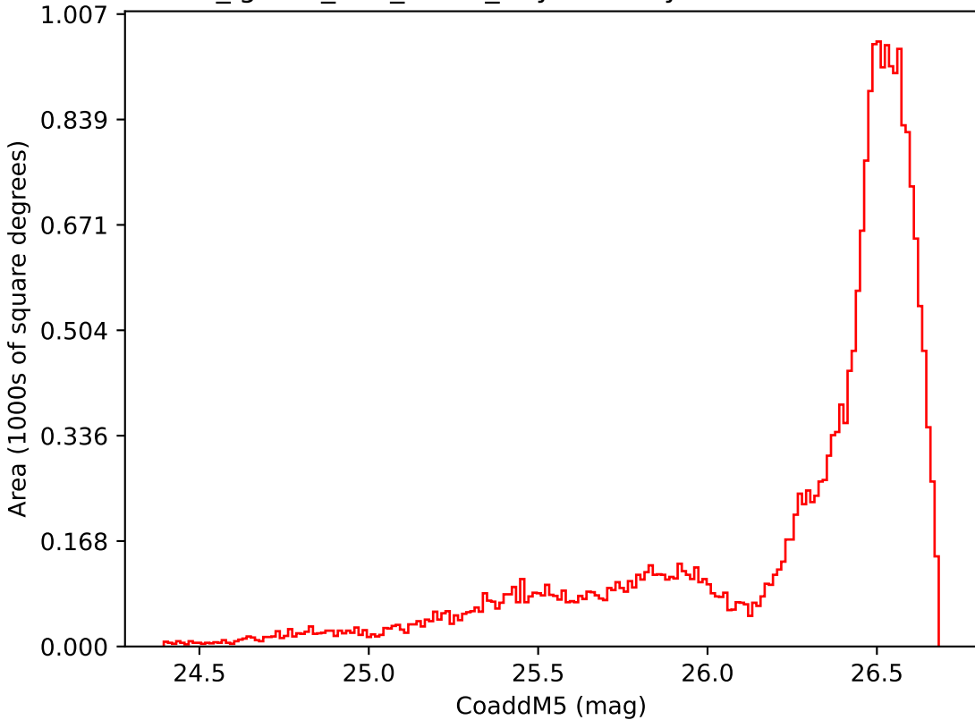
too_ignore_100_1v3.4_10yrs All sky i band: CoaddM5
