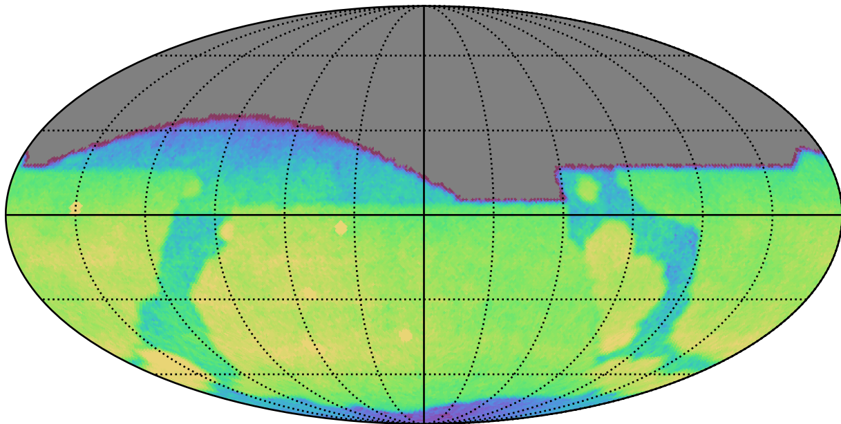
too_ignore_100_1v3.4_10yrs All sky g band: CoaddM5
