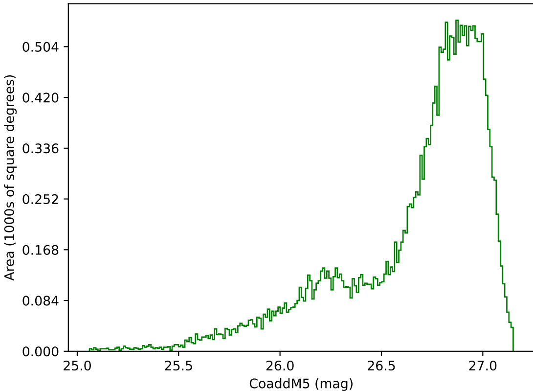
too_ignore_100_1v3.4_10yrs All sky g band: CoaddM5
