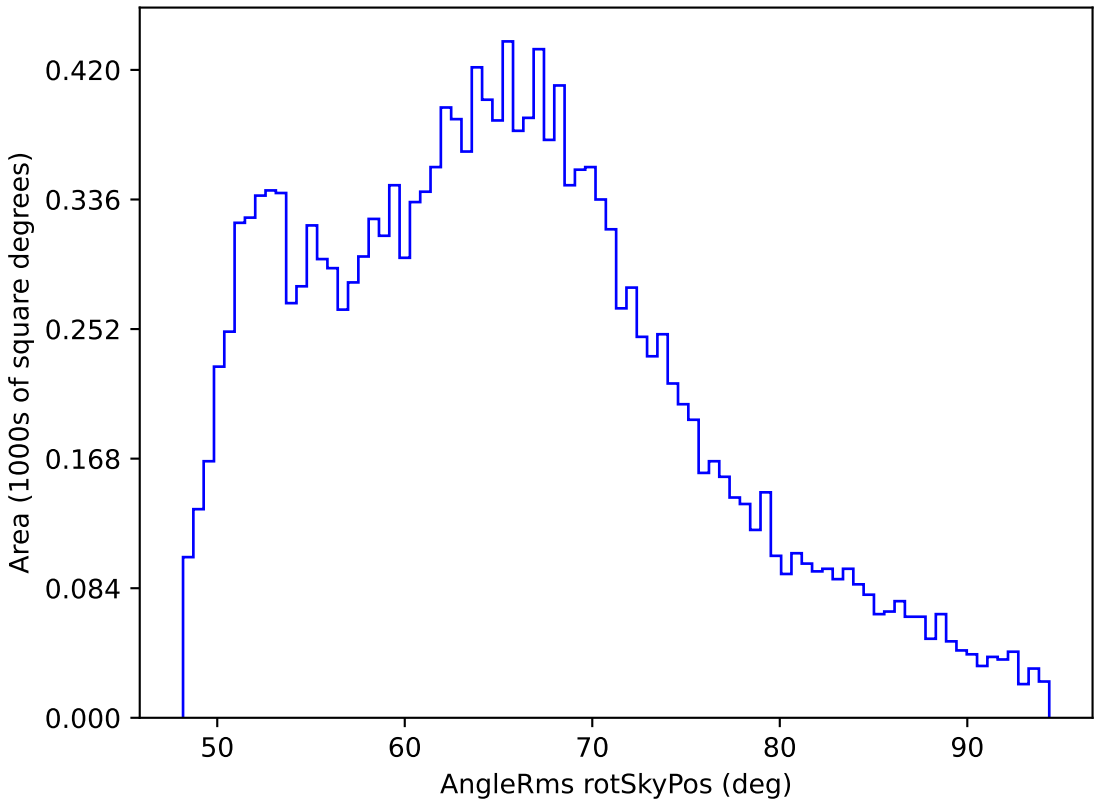
too_ignore_100_1v3.4_10yrs WFD z band: AngleRms rotSkyPos
