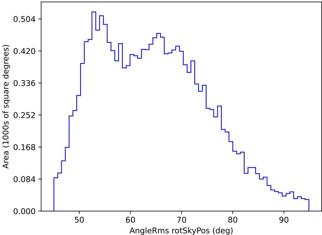
too_ignore_100_1v3.4_10yrs WFD u band: AngleRms rotSkyPos
