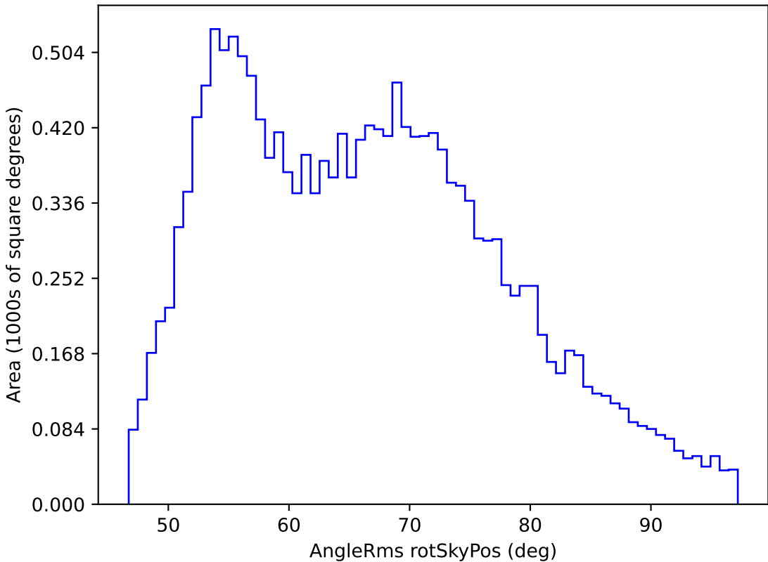
too_ignore_100_1v3.4_10yrs WFD r band: AngleRms rotSkyPos
