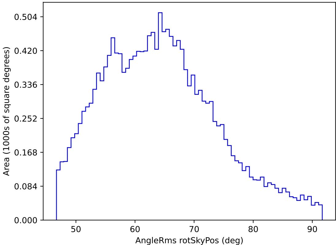
too_ignore_100_1v3.4_10yrs WFD i band: AngleRms rotSkyPos
