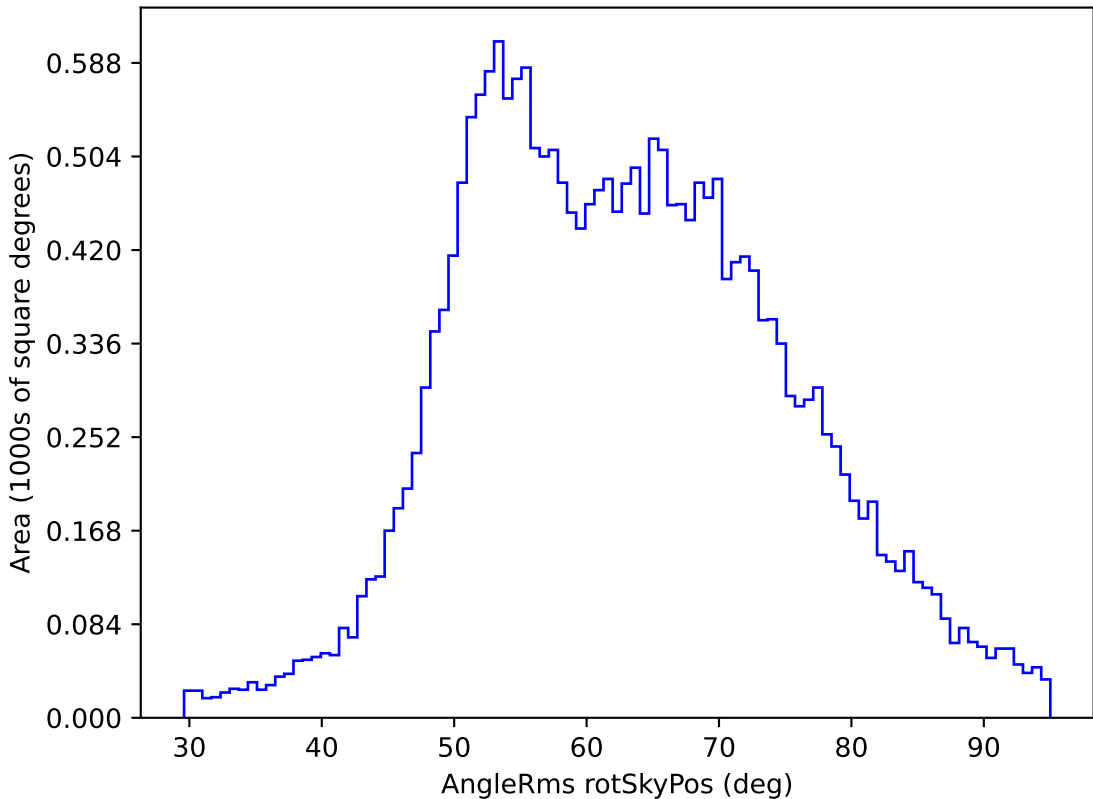
too_ignore_100_1v3.4_10yrs All sky u band: AngleRms rotSkyPos
