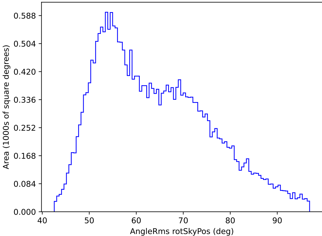
too_ignore_100_1v3.4_10yrs All sky r band: AngleRms rotSkyPos
