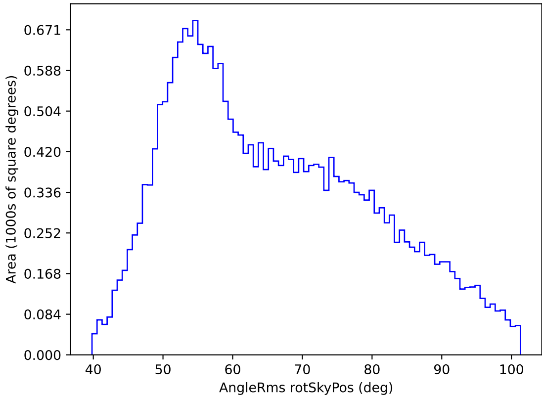
too_ignore_100_1v3.4_10yrs All sky g band: AngleRms rotSkyPos
