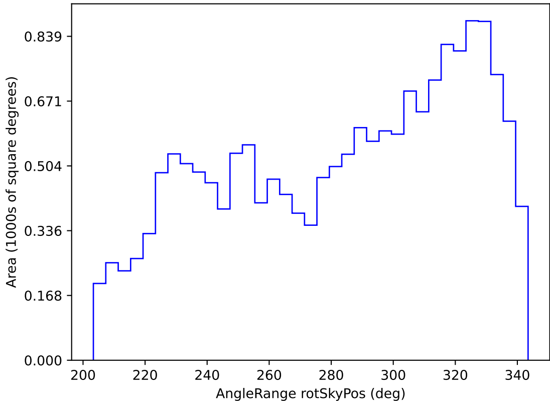
too_ignore_100_1v3.4_10yrs WFD r band: AngleRange rotSkyPos
