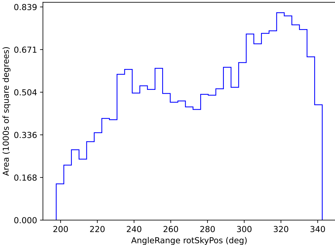
too_ignore_100_1v3.4_10yrs WFD i band: AngleRange rotSkyPos
