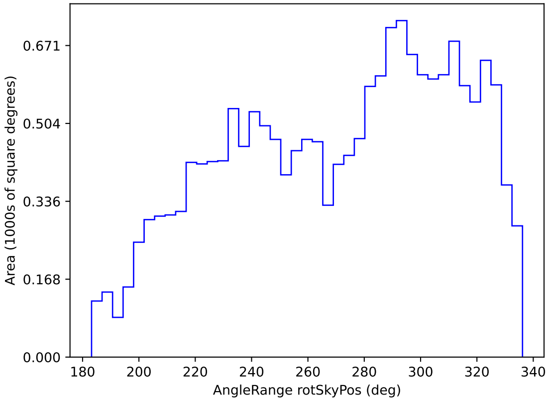
too_ignore_100_1v3.4_10yrs WFD g band: AngleRange rotSkyPos
