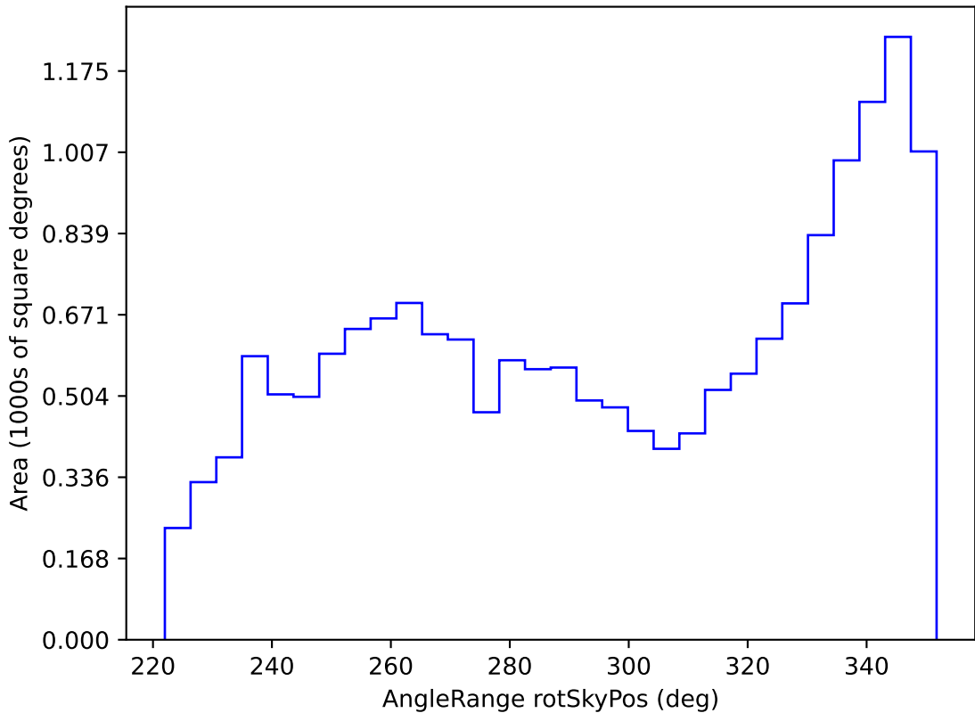
too_ignore_100_1v3.4_10yrs WFD all bands: AngleRange rotSkyPos
