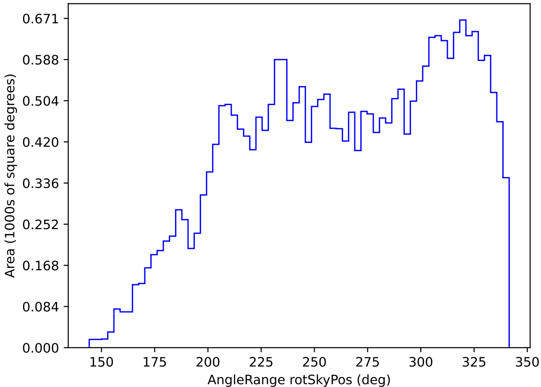
too_ignore_100_1v3.4_10yrs All sky i band: AngleRange rotSkyPos
