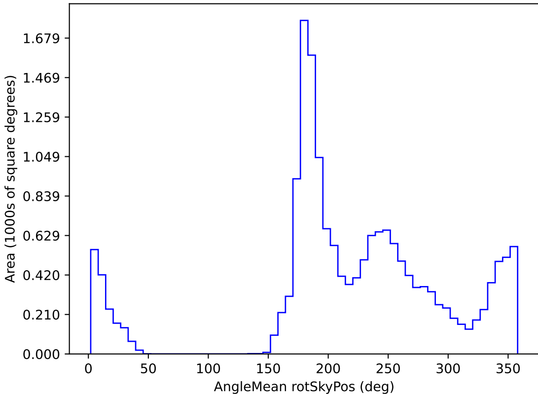
too_ignore_100_1v3.4_10yrs WFD z band: AngleMean rotSkyPos
