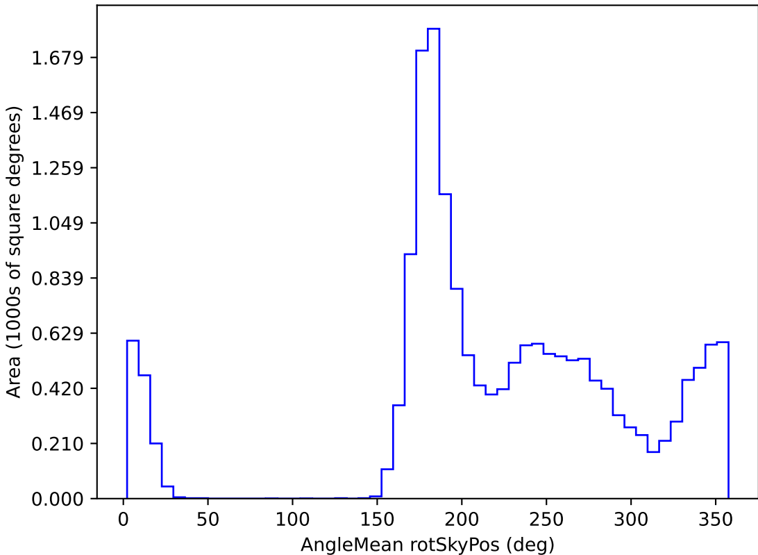
too_ignore_100_1v3.4_10yrs WFD y band: AngleMean rotSkyPos
