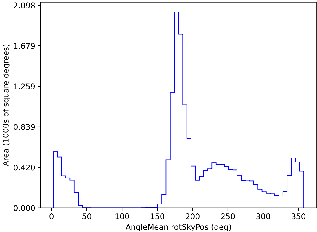
too_ignore_100_1v3.4_10yrs WFD r band: AngleMean rotSkyPos
